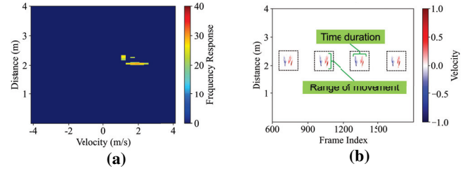
Fig. 4: (a) Doppler-range heatmap after environmental impact mitigation; (b) Spatial-temporal heatmap of four repetitions.
